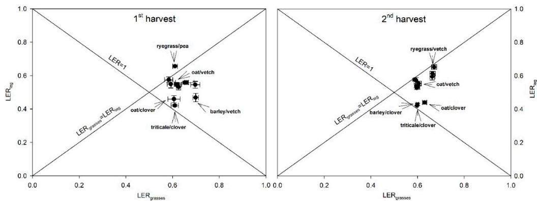
Figure 1. Partial land equivalent ratio calculated for the biomass yield of legumes ( LER_{leg} ) as a function of the partial land equivalent ratio calculated for the biomass yield of grasses ( LER_{grasses} ) in the first and second cuts. Values are the mean ( n = 3 ) \pm SE.
