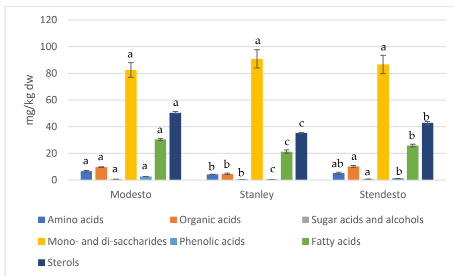
Figure 2. Distribution of chemical classes in studied fruit samples (mg/kg dw). Different letters in the same chemical class indicate statistically significant differences ( p < 0.05 ), according to ANOVA and the Tukey test ( n = 3 ).
