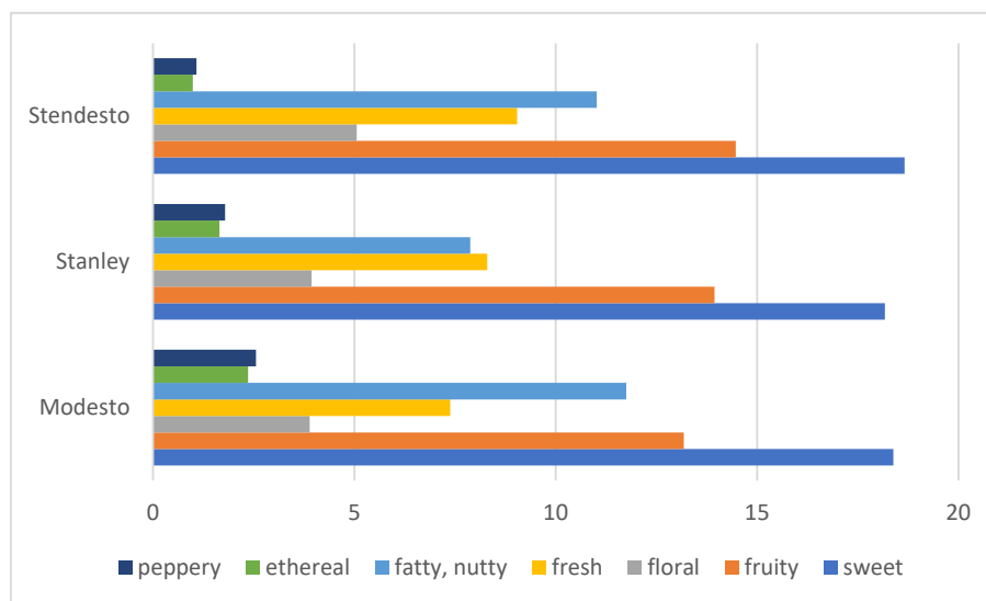
Figure 4. Odor description attribution of VOCs in studied fruit samples ( https://foodb.ca , accessed on 29 December 2023).
