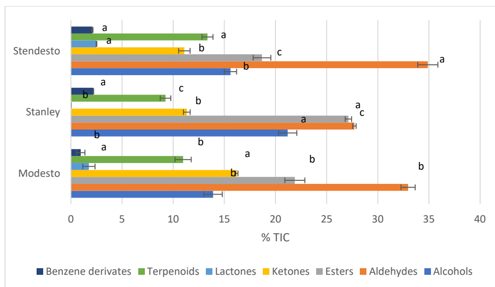
Figure 3. Distribution of VOC chemical classes in studied fruit samples (%TIC). Different letters in the same chemical class indicate statistically significant differences ( p < 0.05 ), according to ANOVA and the Tukey test ( n = 3 ).
