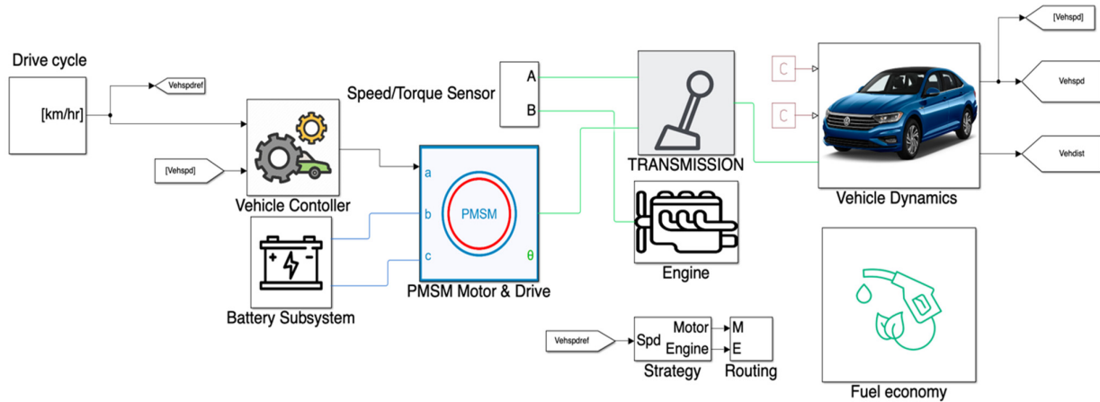
Figure 12. Parallel hybrid powertrain MATLAB model.
