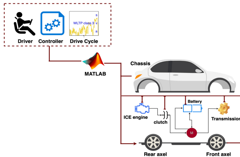
Figure 4. Model-in-the-loop testing for the hybrid vehicle.
