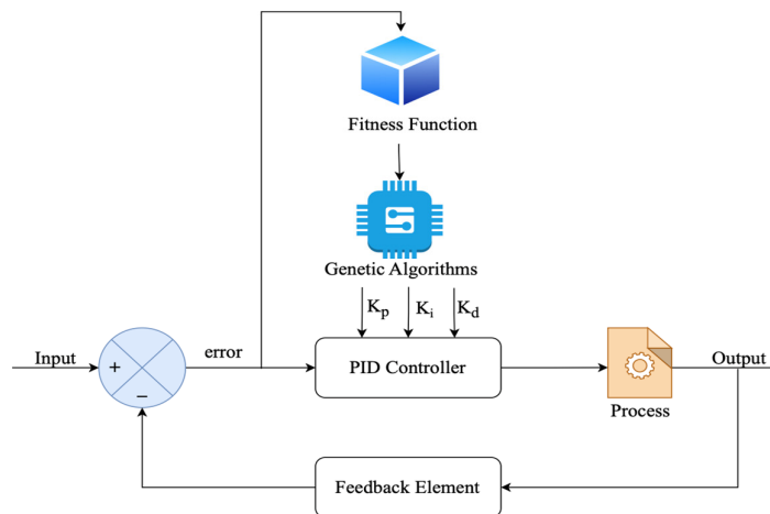
Figure 7. GA-PID configuration.
