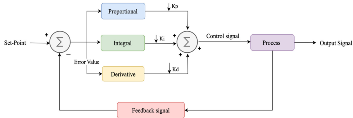
Figure 6. PID control action.
