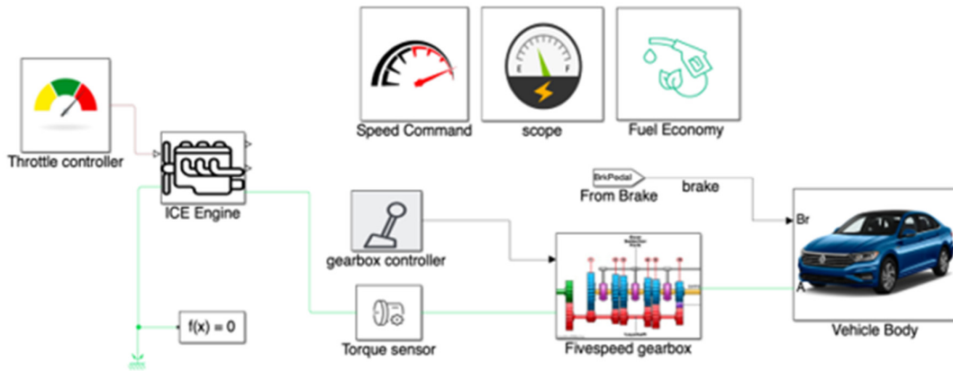
Figure 11. Conventional MATLAB model.
