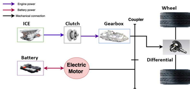
Figure 3. Configuration of the hybrid powertrain.
