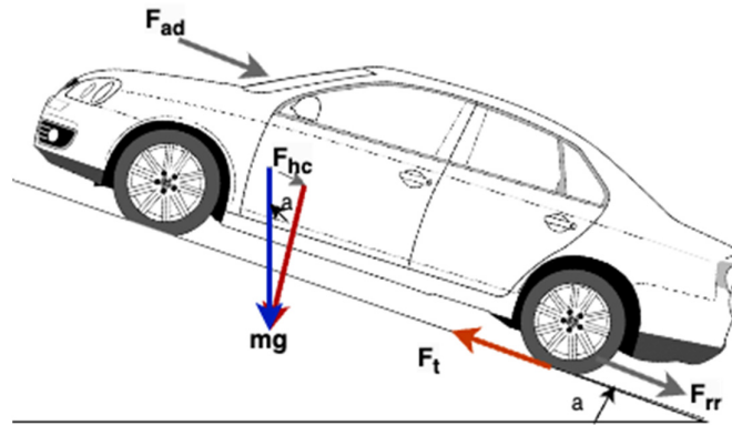
Figure 1. Free body diagram of the vehicle dynamics.
