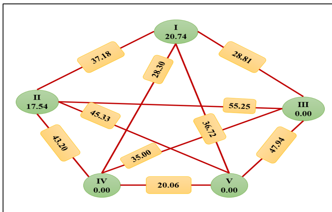
Fig. 3. Cluster diagram based on D 2 statistics
