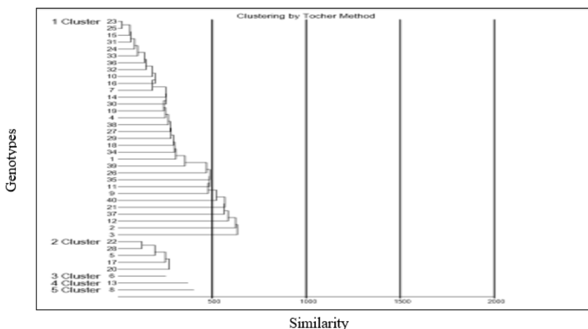
Fig. 2. Dendrogram of forty rice genotypes for fourteen characters
