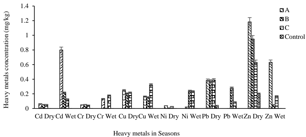
Fig. 2. Mean Concentration of heavy metals at the sampling points during dry and wet seasons
