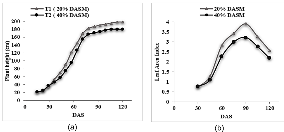
Fig. 2. (a) Plant height and (b) leaf area index of maize crop as influenced by different irrigation treatments during rabi, 2022-23.
