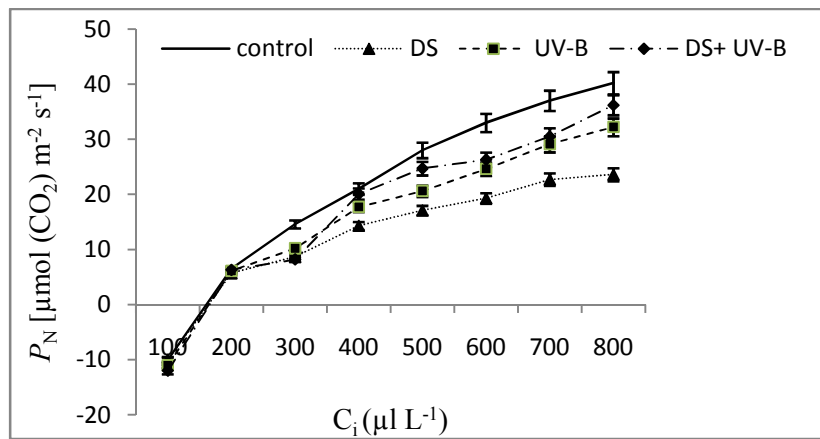
Fig. 4. Photosynthetic response to internal \text{CO}_2 partial pressures ( C_i ) for lettuce subjected to drought stress and UV-B singly and in combination. ( n = 10 \pm 1 SE).
