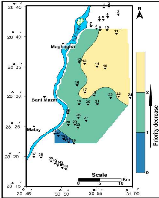
Fig. 25: Priority Map for Samalut Aquifer.
