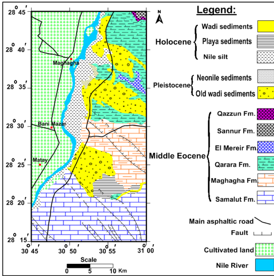
Fig. 3: Geological Map of the Study Area (After EGSMA et al, 2005)
