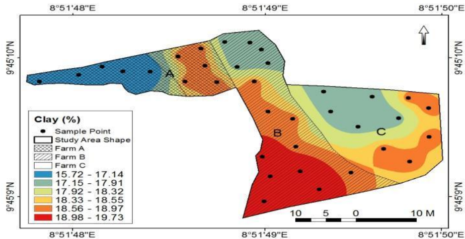
Fig. 12. Surface distribution of Clay
