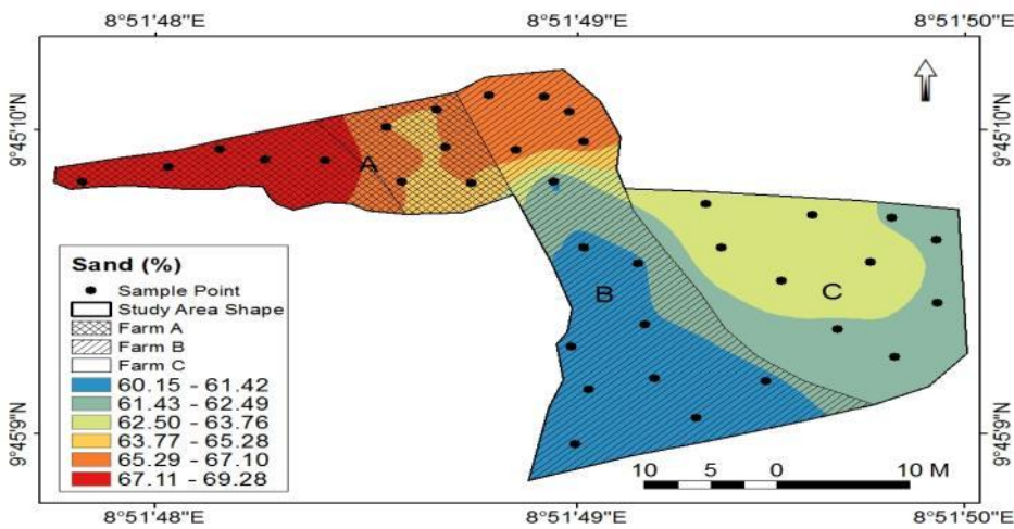
Fig. 10. Surface distribution of Sand
