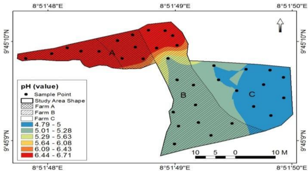
Fig. 2. Surface distribution of pH
