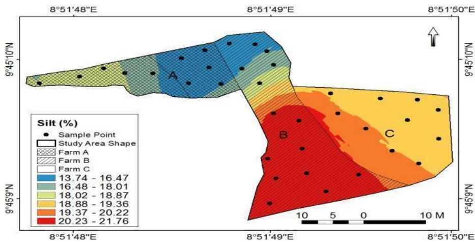
Fig. 11. Surface distribution of Silt
