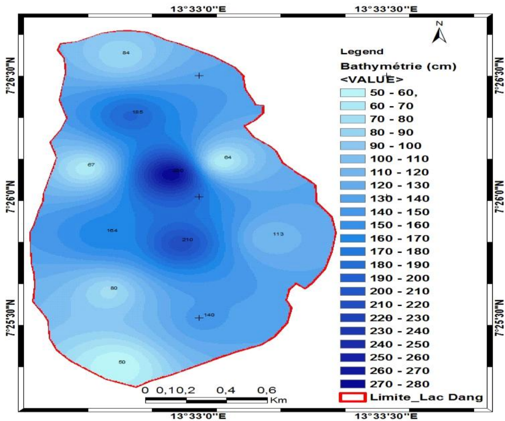
Fig. 8. Bathymetry of Lake Dang
