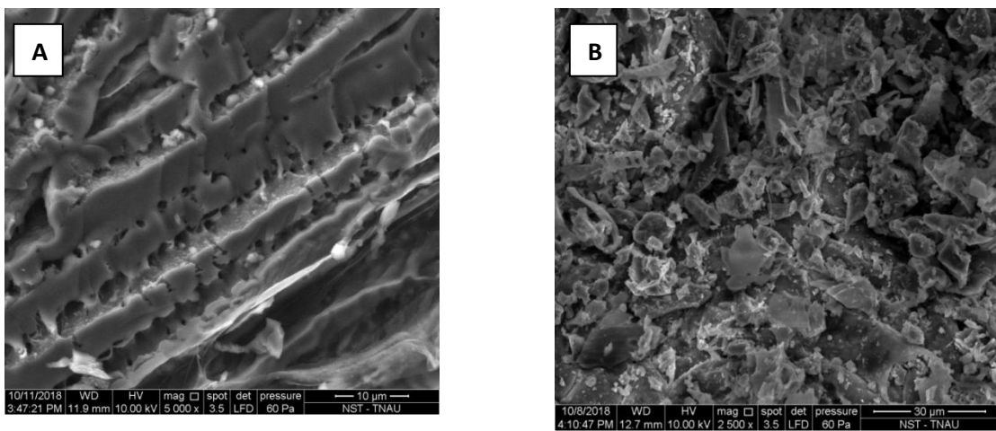
Fig. 2. SEM images of Vetiver (A) and Vermiculite (B)
