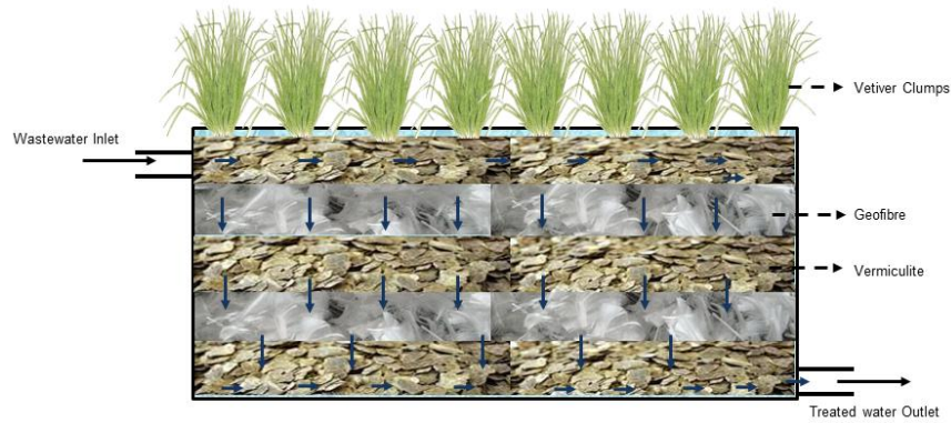
Fig. 1. Pilot scale Vetiver Constructed wetland setup for Wastewater treatment
