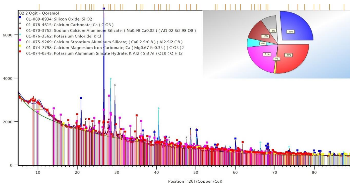
Fig. 4. X-ray analysis of the inorganic part of the sample of organomineral fertilizer obtained in the ratio CM:NB:FF:NFM=100:5:2.5:4
