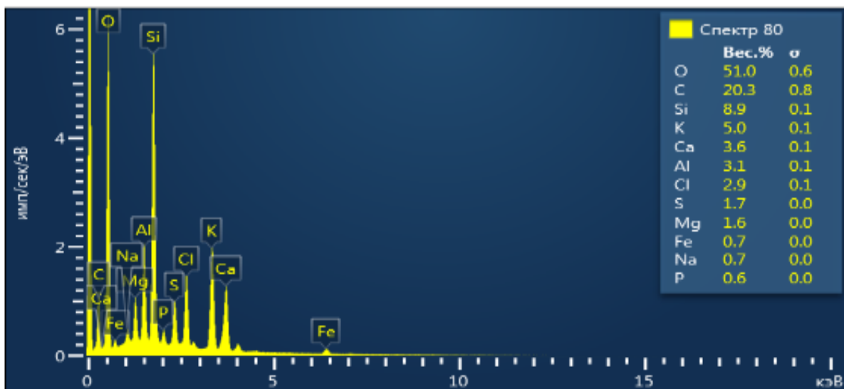
Fig. 3. CM:NB:FF:NFM=100:5:2.5:4 elemental composition of the organomineral fertilizer sample taken in proportion
