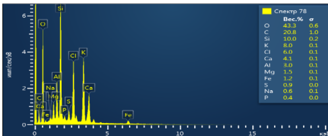
Fig. 1. Elemental composition of the organomineral fertilizer sample obtained in the ratio CM:NB:NFM=100:2.5:4
