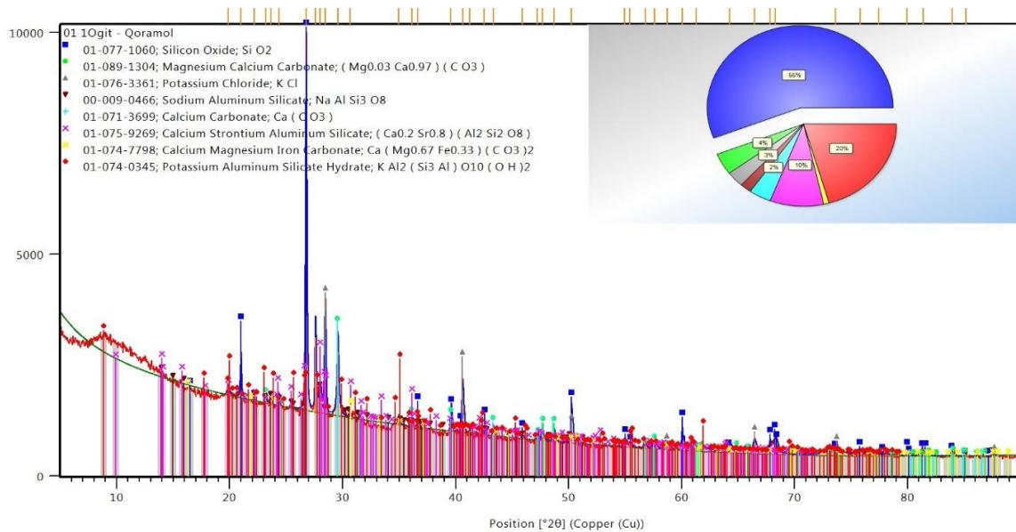
Fig. 2. X-ray analysis of the inorganic part of the sample of organomineral fertilizer obtained in the ratio CM:NB:NFM =100:2.5:4
