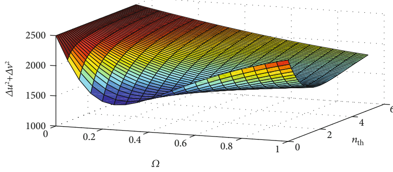
FIGURE 9: A plot of the atom entanglement of the two-mode cavity light (Equation (44)) versus \Omega and \bar{n}_{\text{th}} for \gamma_c = 0.4 and \gamma = 0.2 (color online) N = 50 .
