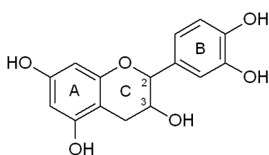
Fig. 4. Chemical structure of Flavonoids
