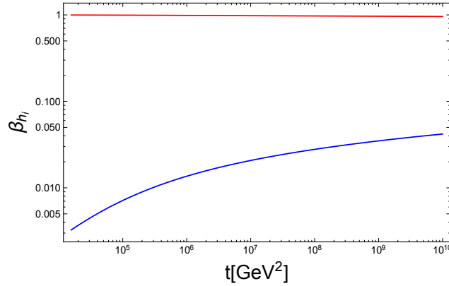
Fig. 6. Splitting fractions of the Higgs cubic (red) and quartic (blue) interactions. Notice that \beta_{3h} + \beta_{4h} = 1 . The plot shows that for moderate energies the cubic splitting dominates over the quartic one, while the quartic only begins to dominate at energies \gtrsim 8 \times 10^{134} GeV (not shown on the plot), see Eq. (39). The plot is on a log-log scale.
