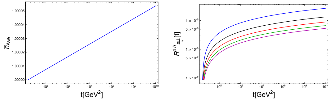
Fig. 5. (Left): The quartic Higgs average jet multiplicity with the energy scale. (Right): The quartic Higgs jet scaling pattern given in Eq. (37c), with n = 1 (blue), n = 2 (gray), n = 3 (red), n = 4 (green), n = 5 (magenta). The plot clearly shows a Poisson scaling pattern (see Eq. (32)). Both plots are on a log-log scale
