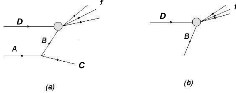
Fig. 1. Factorization of the 3-vertex splitting
