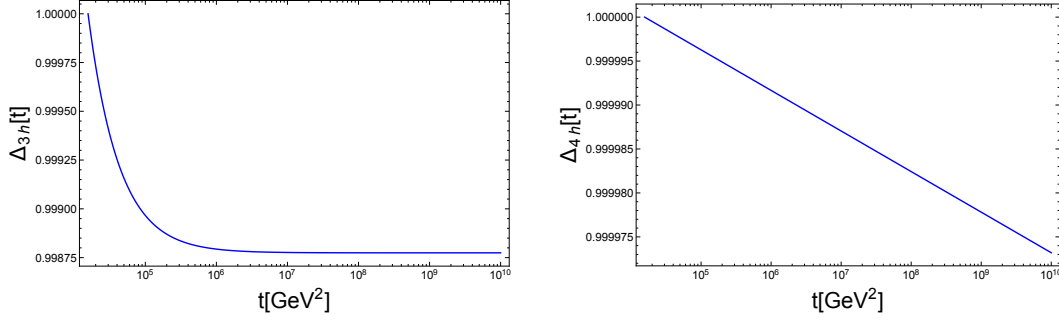
Fig. 2. (Left): The cubic Higgs Sudakov factor as a function of the virtuality t . (Right): The quartic Higgs Sudakov factor. The plots are on a log-log scale
