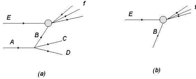
Fig. 3. Factorization of the 4-vertex splitting
