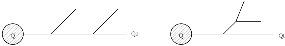
Fig. 7. Primary emission (left) vs. secondary emission (right)
