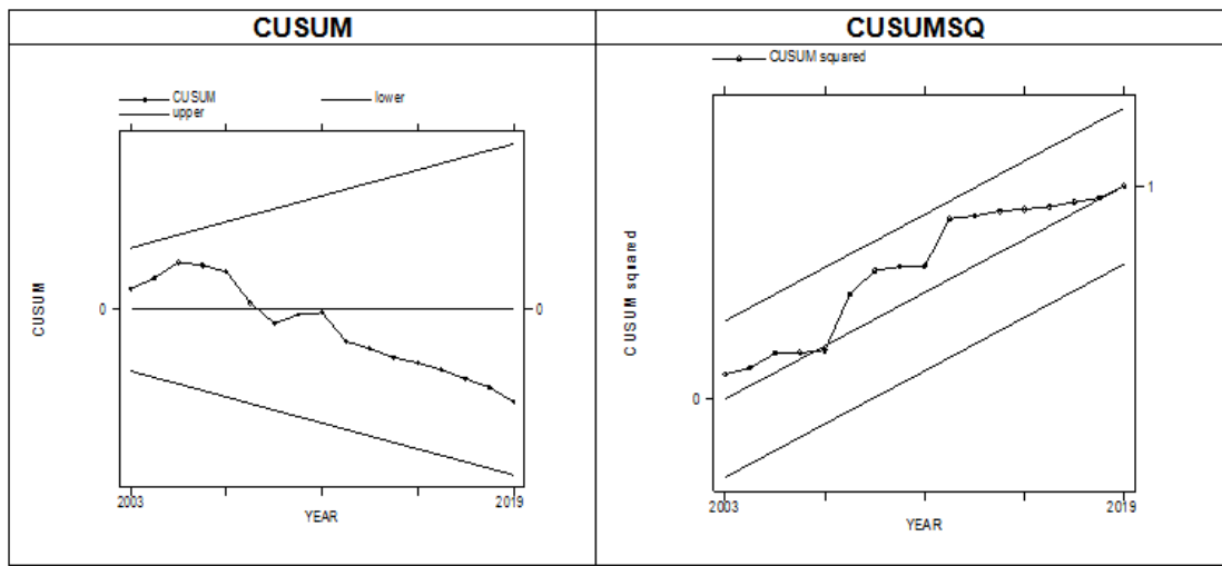
Fig. 1. Plot of recursive and squared recursive residuals against breakpoints
