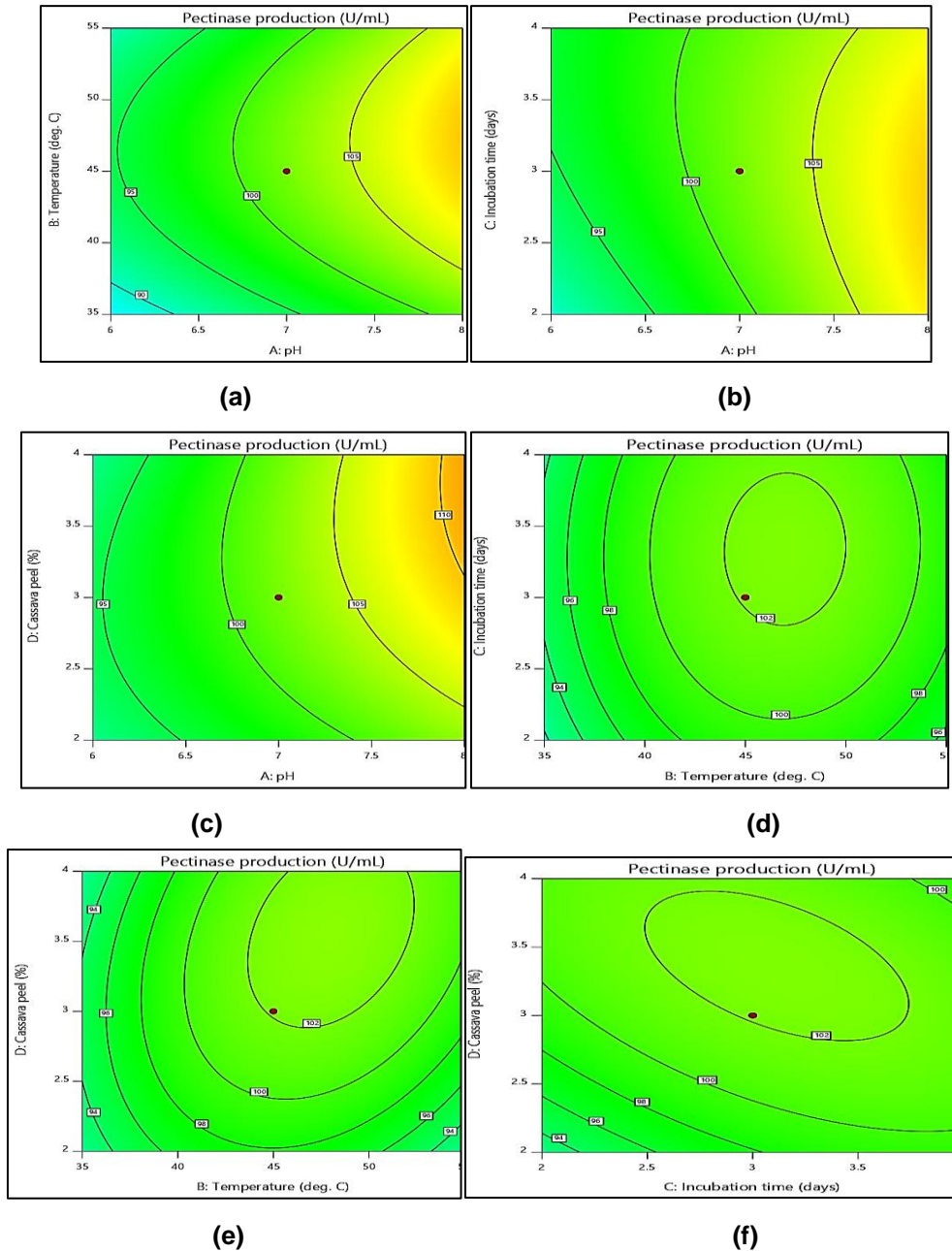
Fig. 1. Response surface plots for pectinase production (U/mL) from B. subtilis PSE-8 through submerged fermentation as a function of (a) pH and temperature (°C) (b) pH and incubation time (c) pH and cassava peel concentration (d) temperature and incubation time (e) temperature and cassava peel concentration (f) cassava peel concentration and incubation time
