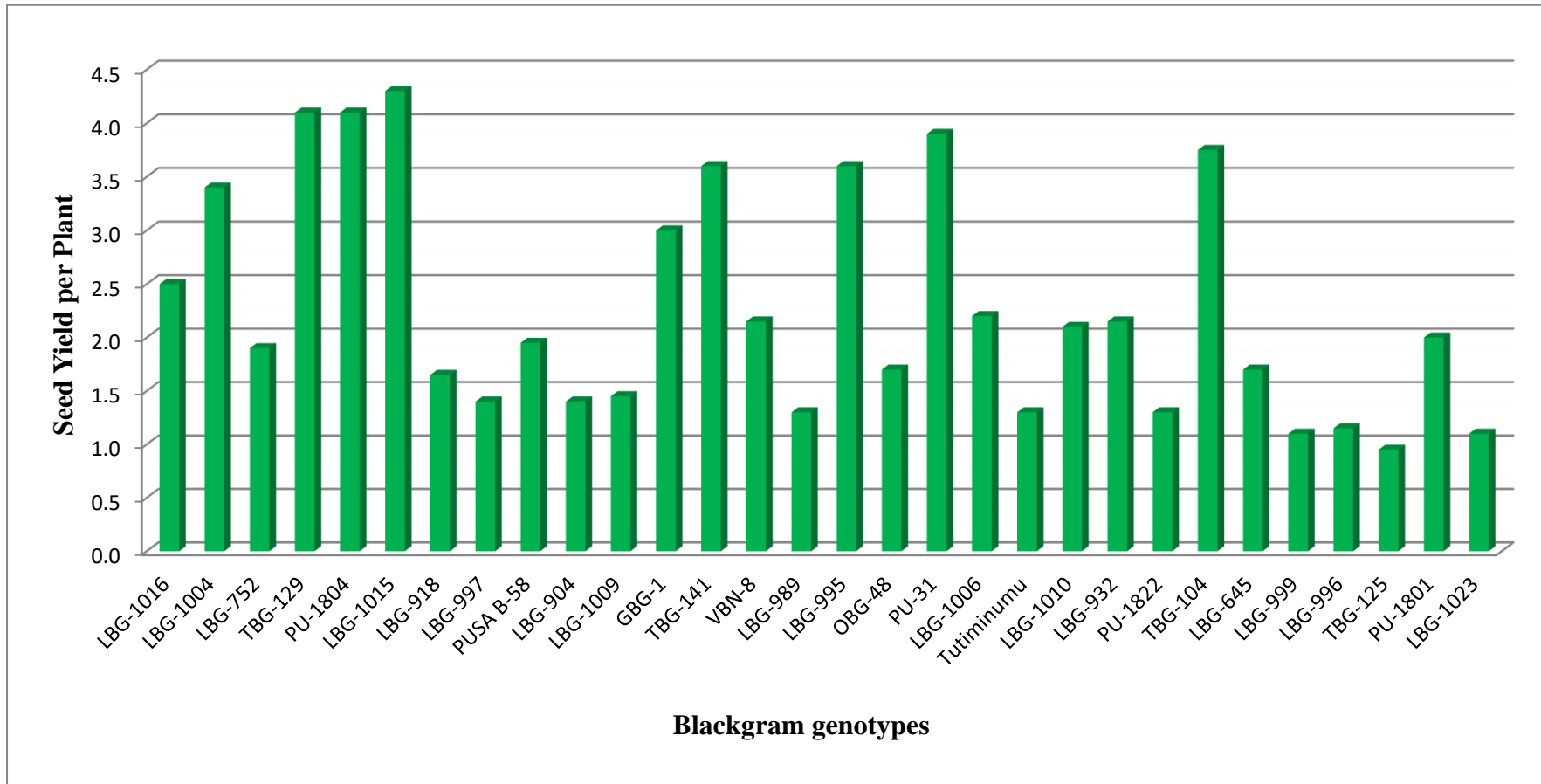
Fig. 4. Effect of high temperature stress on seed yield per plant (g plant -1 ) of blackgram genotypes at pod formation stage (pooled data)
