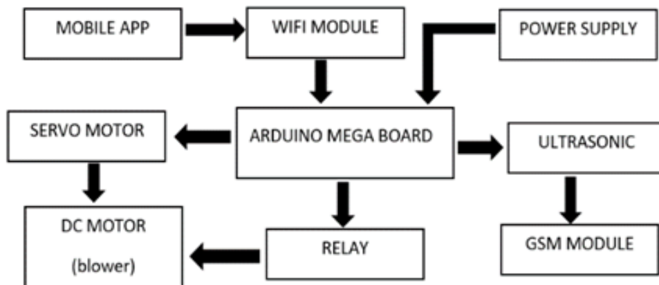
Fig. 2. Block diagram of the project
