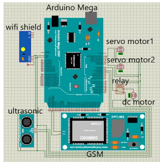
Fig. 15. Schematic diagram
