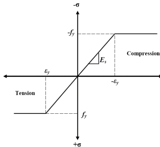
Fig. 5. Idealized stress-strain curve for reinforcing steel
