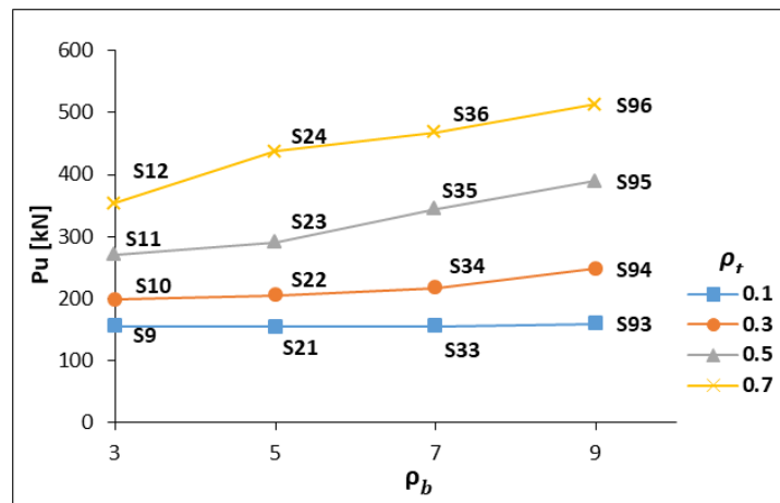
Fig. 11. Variation of ultimate load P_u with flange width ratio ( \rho_b ) at different flange thickness ratios ( \rho_f ) for \rho = 0.5 , f_c' = 30 MPa & a/h = 2
