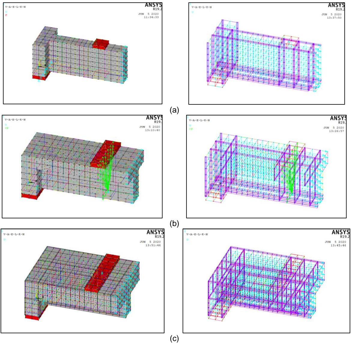
Fig. 8. Finite Element Simulation Models for specimens: a) Rectangular; b) G1-0.3-3; and c) G3-0.5-5 from Ref. [16]
