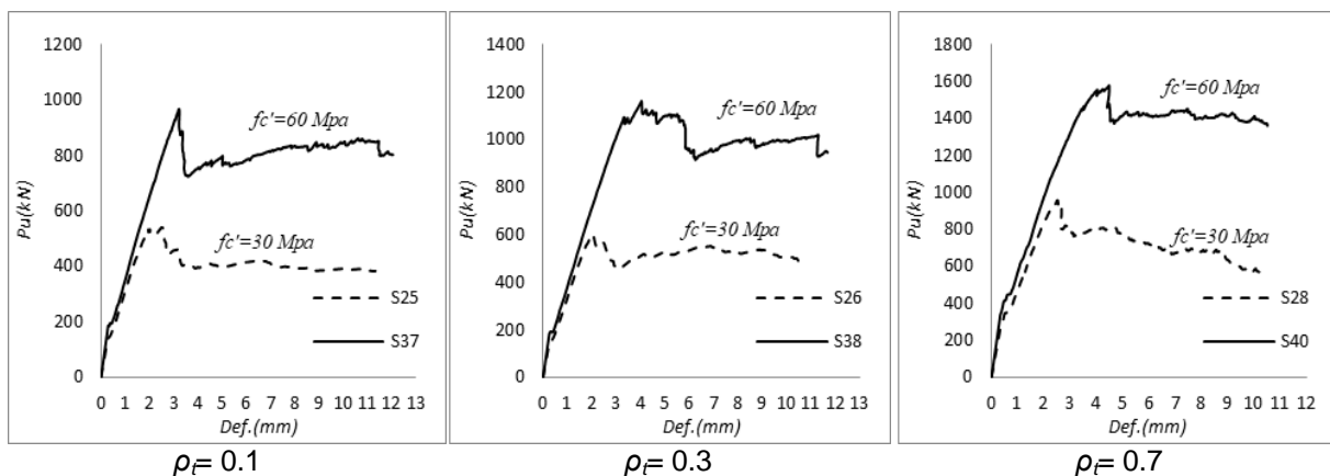
Fig. 18. Effect of concrete characteristic strength on load-deflection relationship for beams with variable flange thickness ( \rho_b=7, a/h=0.5 )
