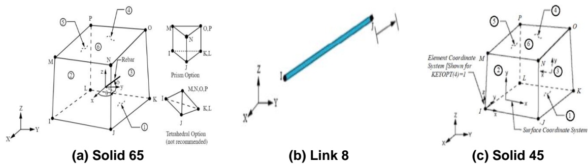
Fig. 1. Structural elements idealization for the numerical models [9]
