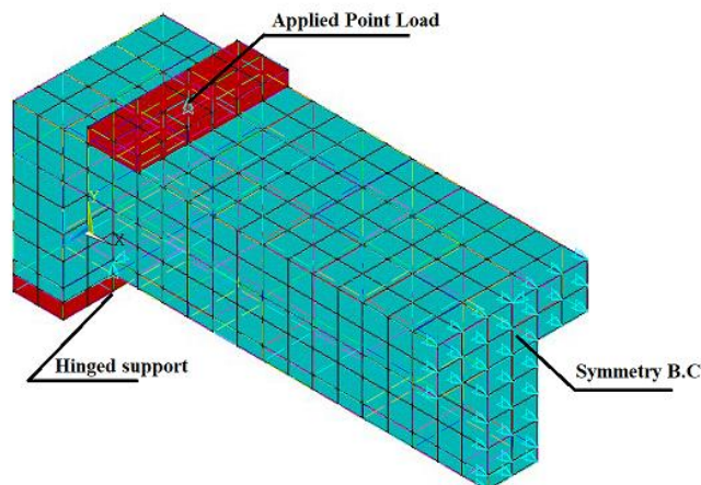
Fig. 2. Applied load and support conditions
