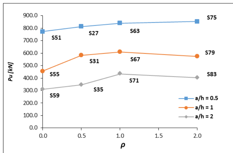
Fig. 13. Effect of flange longitudinal reinforcement on Ultimate load for different shear span to depth ratios for \rho_b = 7 , \rho_t = 0.5 & f_c' = 30 MPa
