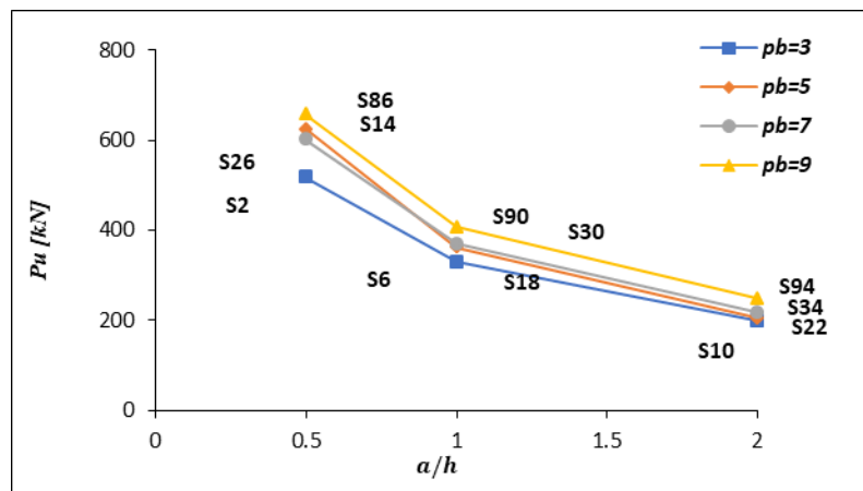
Fig. 15. Effect of shear span-to-depth ratio on ultimate shear strength of T-beams with various flange widths ( \rho_t = 0.3, \rho = 0.5 & f_c' = 30 MPa)
