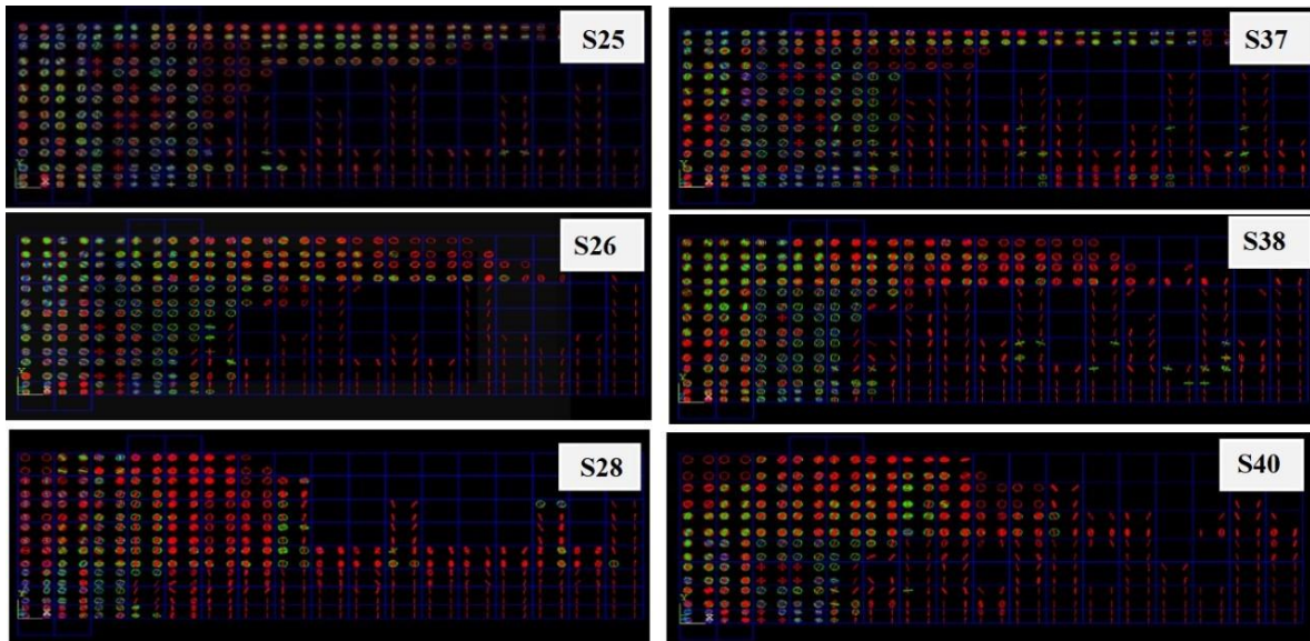
Fig. 19. Effect of concrete characteristic strength on crack patterns at failure for beams with variable flange thickness: \rho_f=0.1 for S25&37, 0.3 for S26&38, 0.7 for S28&40 ( \rho_b=7 , a/d=0.5 & \rho=0.5\% )
