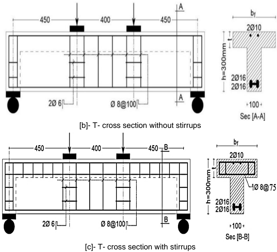
Fig. 6. Specimen details and arrangement of reinforcement (All dimensions in mm) [16]
