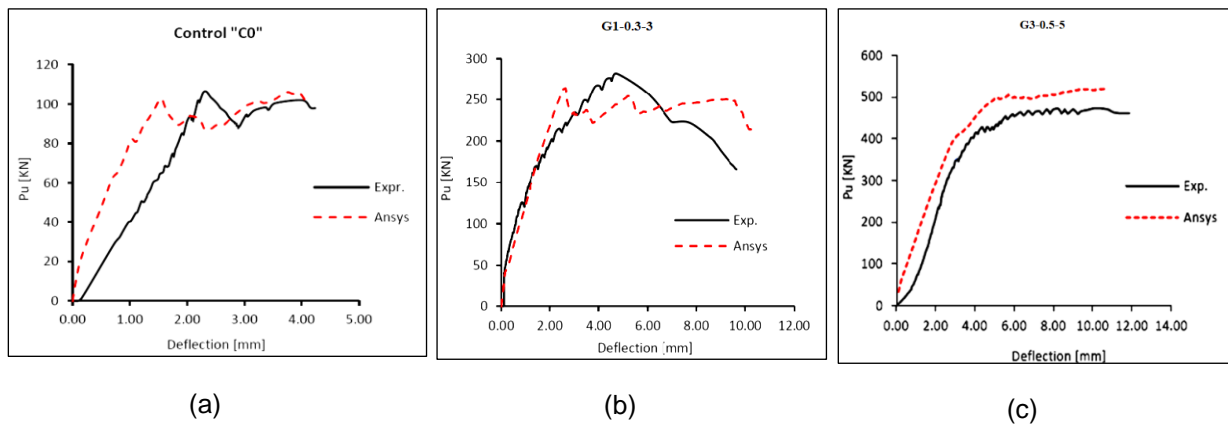
Fig. 9. Predicted and Measured Load-Deflections Curves for Three Specimens: a) Rectangular; b) G1-0.3-3; and c) G3-0.5-5. [16]
