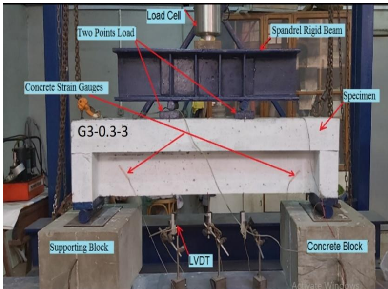
Fig. 7. Preparation of Test Set-up Specimens [16]
