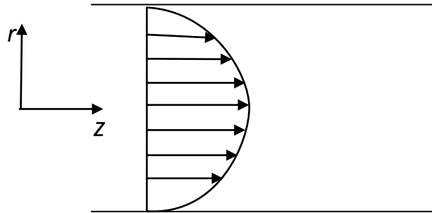
Fig. 3. The velocity profile of blood plasma through a cross section of a non-deformed artery
