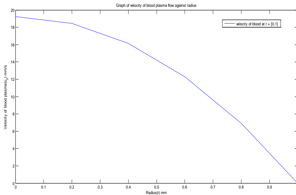
Fig. 2. Variation of axial velocity of blood plasma ( u_z ) with radius of artery ( r )
