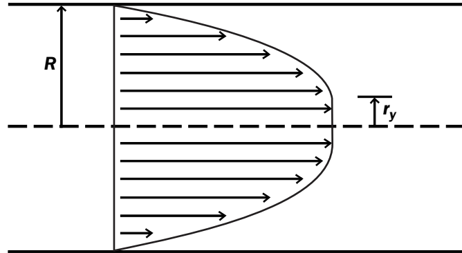
Fig. 1. The velocity profile of blood flowing through a cylindrical vessel using the Casson model. The profile is blunter than a purely Newtonian fluid’s velocity profile because the fluid that is between the centreline and r_y flows as a solid. At r_y , the shear stress ( \tau ) exceeds the yield stress ( \tau_y ) and the viscous forces take effect.
